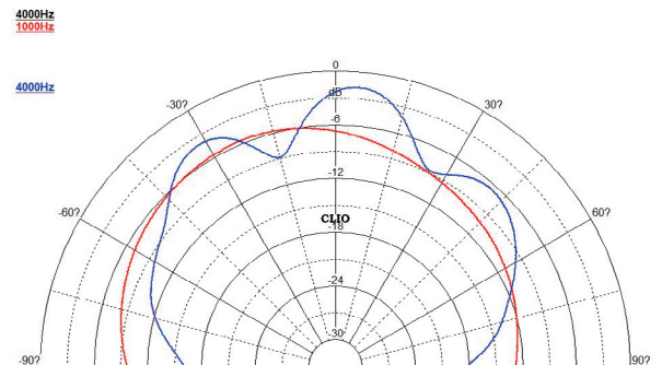
Polar Pattern(V)
