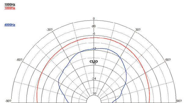
Polar Pattern(H)
