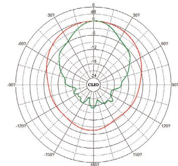
Polar Pattern(V)
