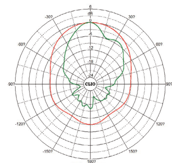
Polar Pattern(H)
