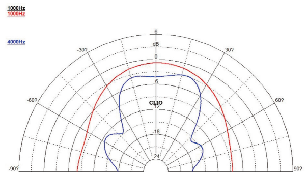
Polar Pattern
